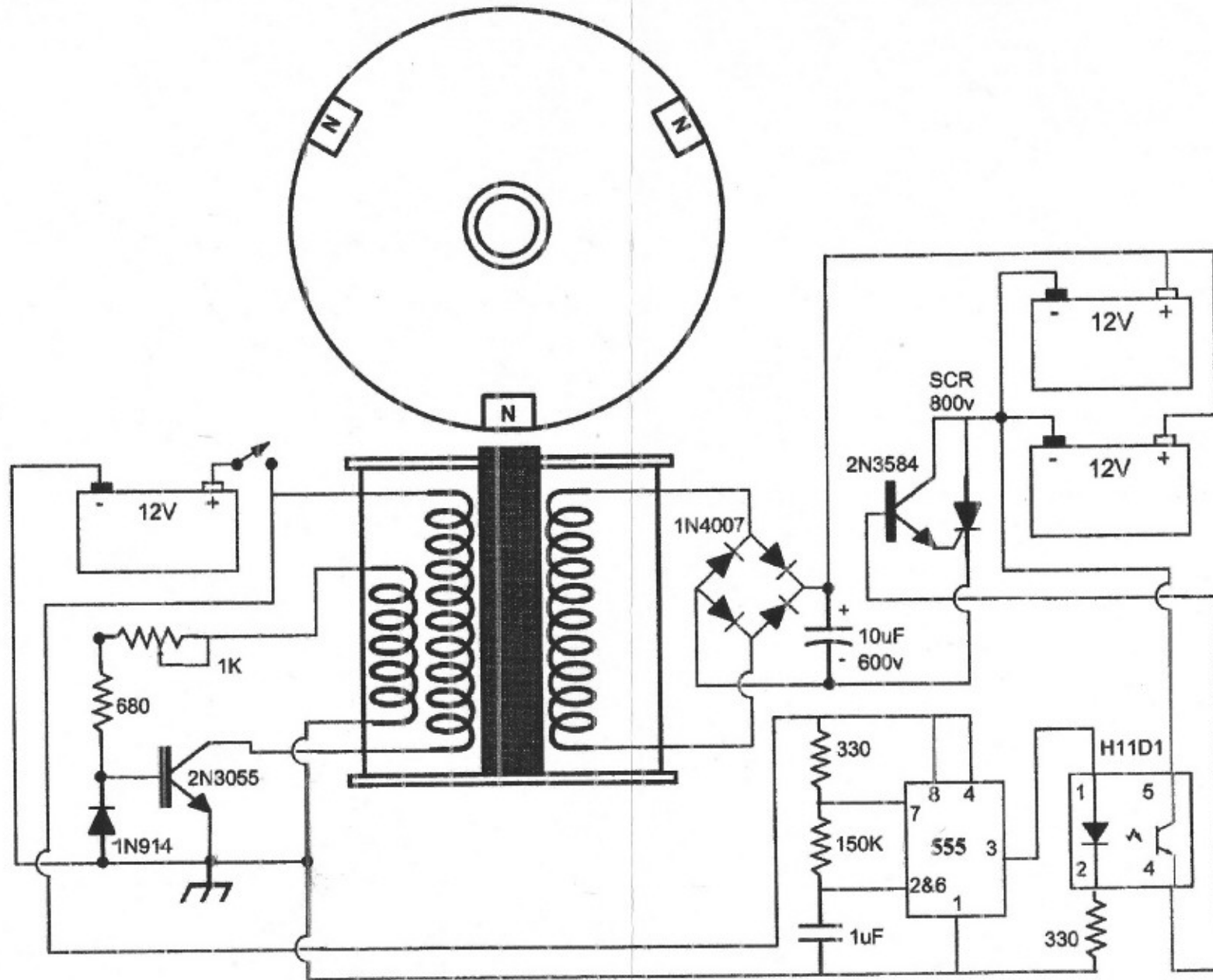
FIGURE 24. RADIANT ENERGY POWERING OF THE MONOPOLE MOTOR
